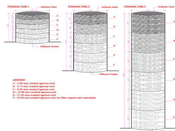
Fig.2. Designed Experimental Filters Indicating the Various Layers
